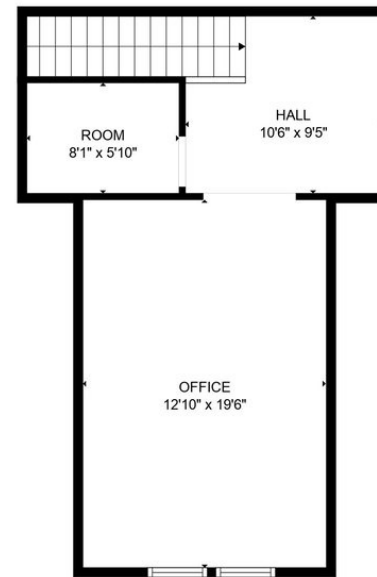
FLOOR 2
