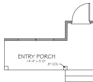
OPTION: FRONT PORCH ADDS 63 UNHEATED SQ. FT. REQUIRES ELEVATION B
