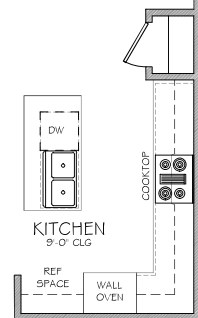
OPTION: KITCHEN
