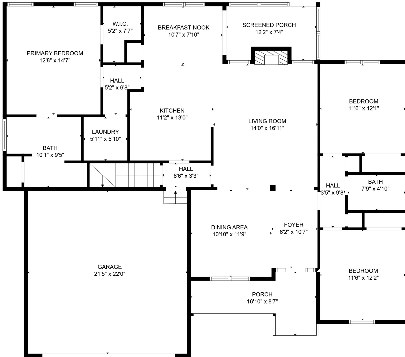
FLOOR 1
