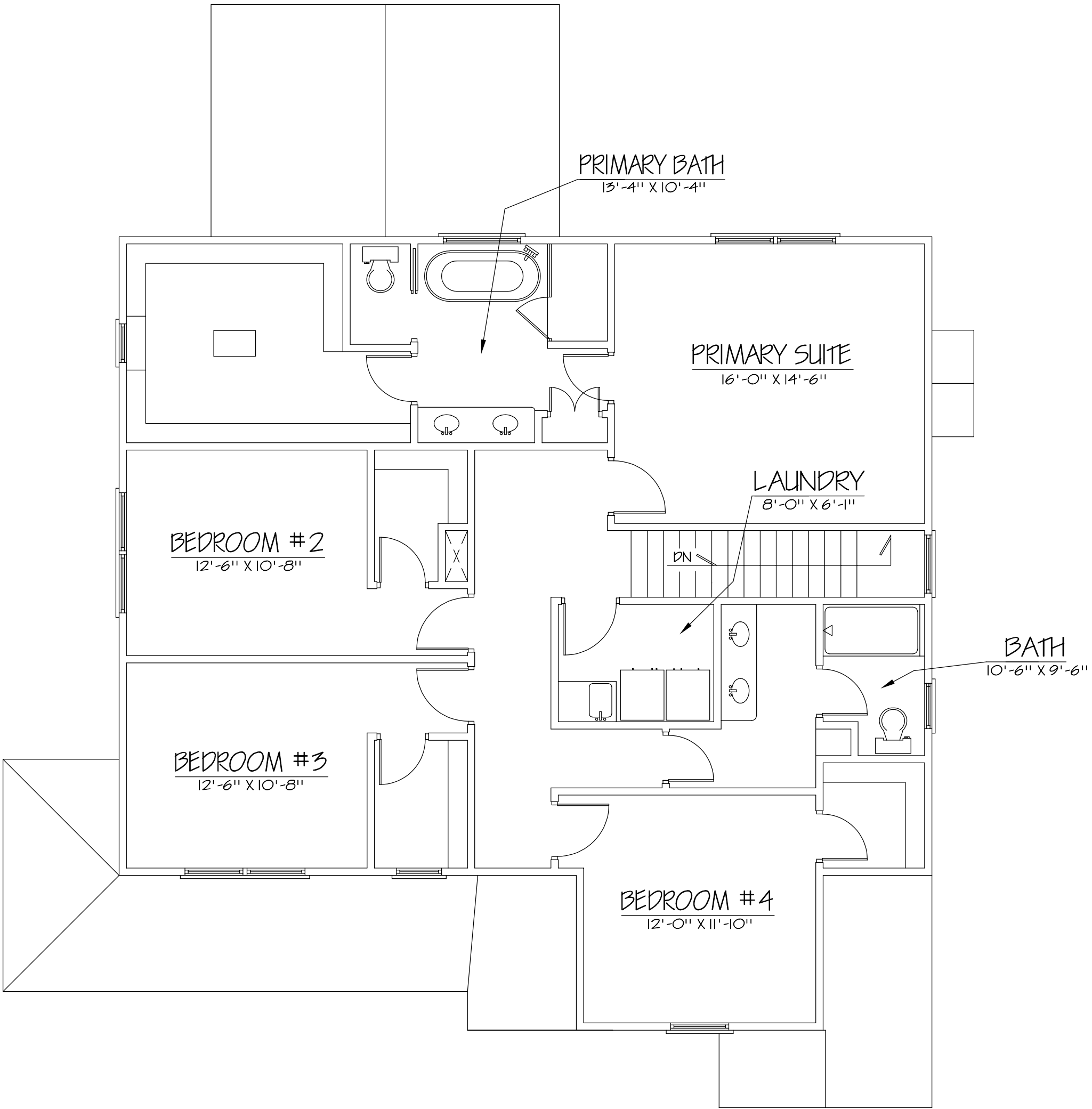
FRONT SECOND FLOOR PLAN
