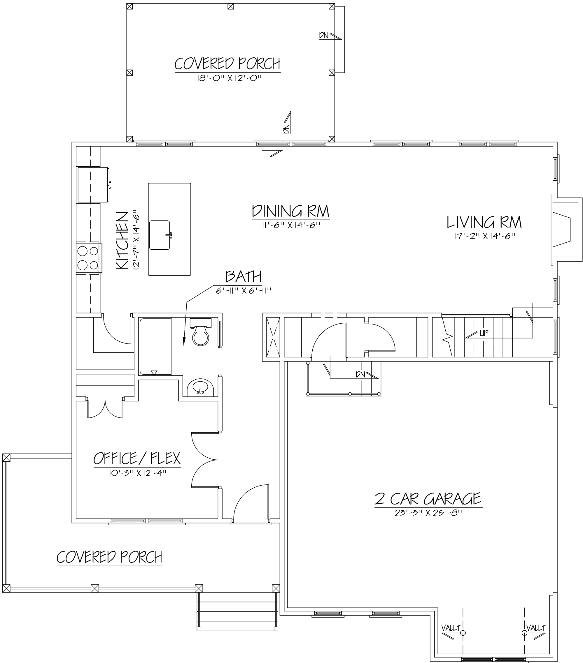
FRONT FIRST FLOOR PLAN
