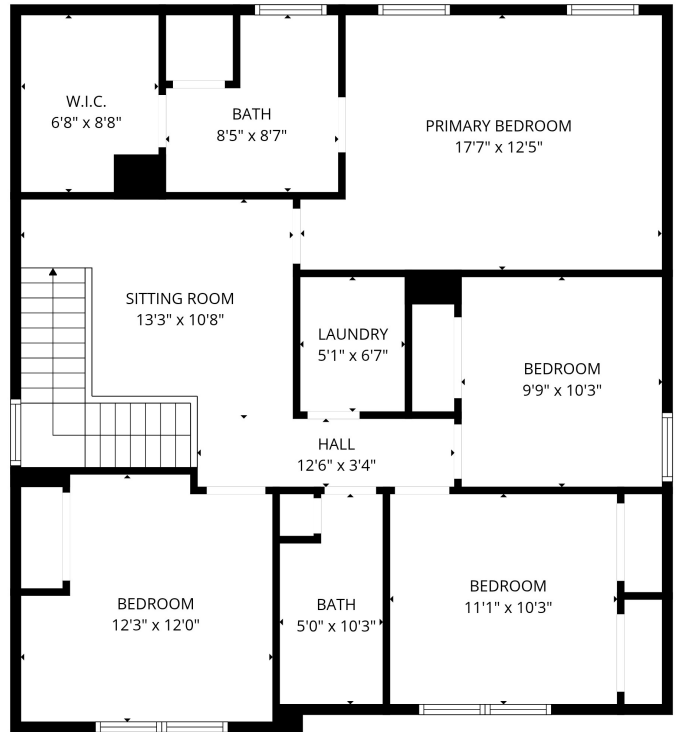
2nd floor
