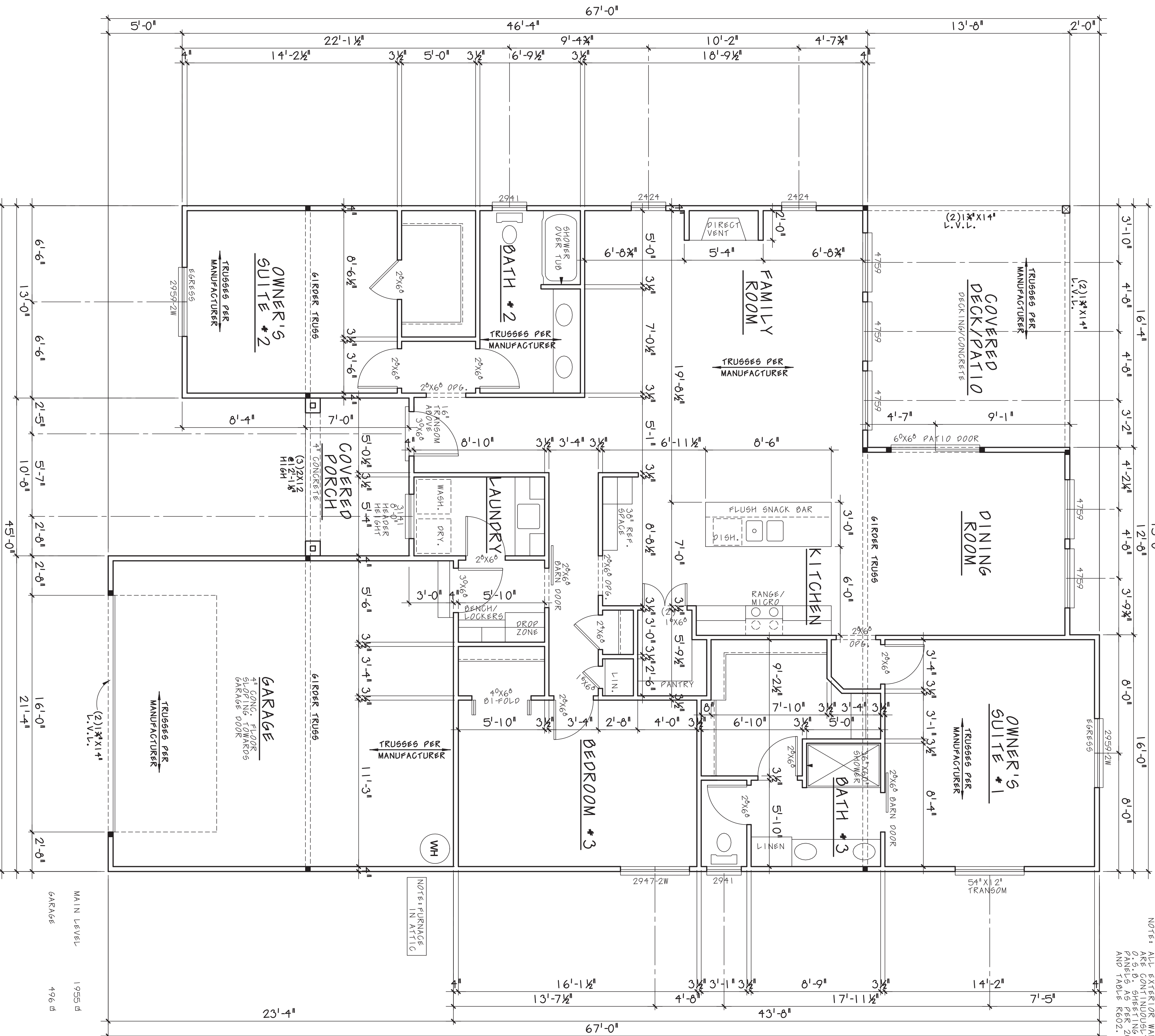
MAIN LEVEL FLOOR PLAN SCALE: 1/4" = 1'-0"
