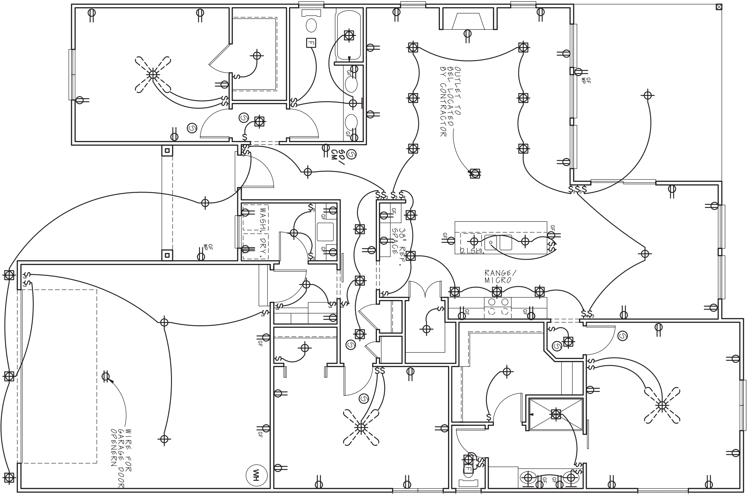
MAIN LEVEL ELECTRICAL SCALE: 3/16" = 1'-0"
