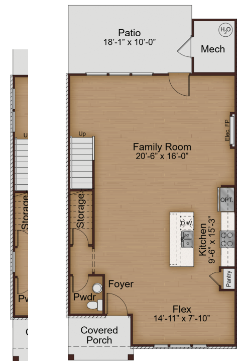
First Floor "A"
