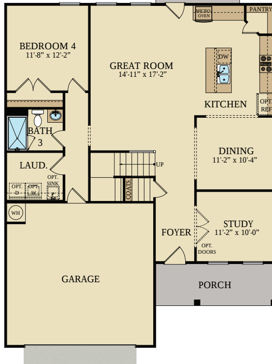
MAIN LEVEL FLOOR PLAN
