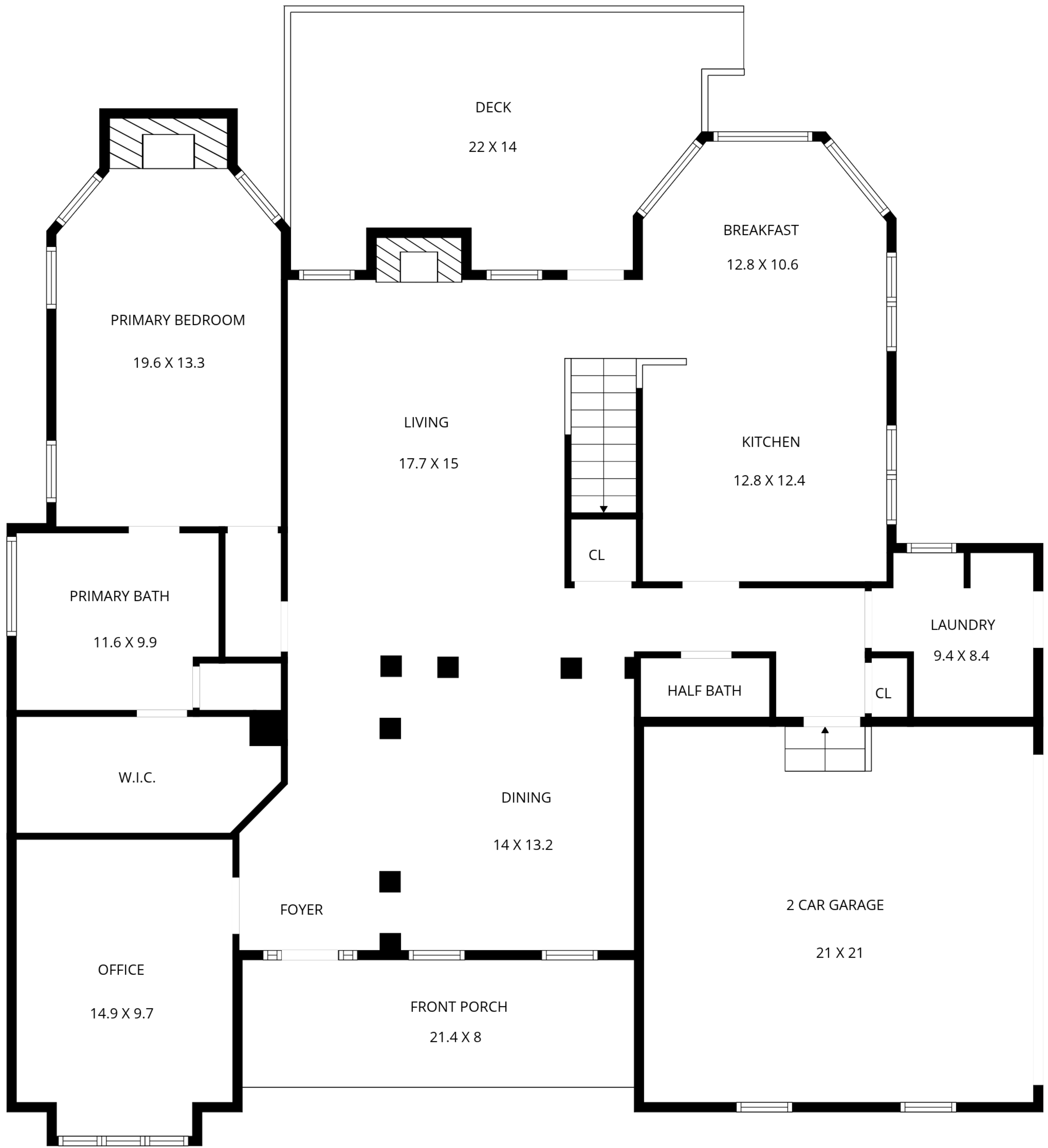
1st floor
