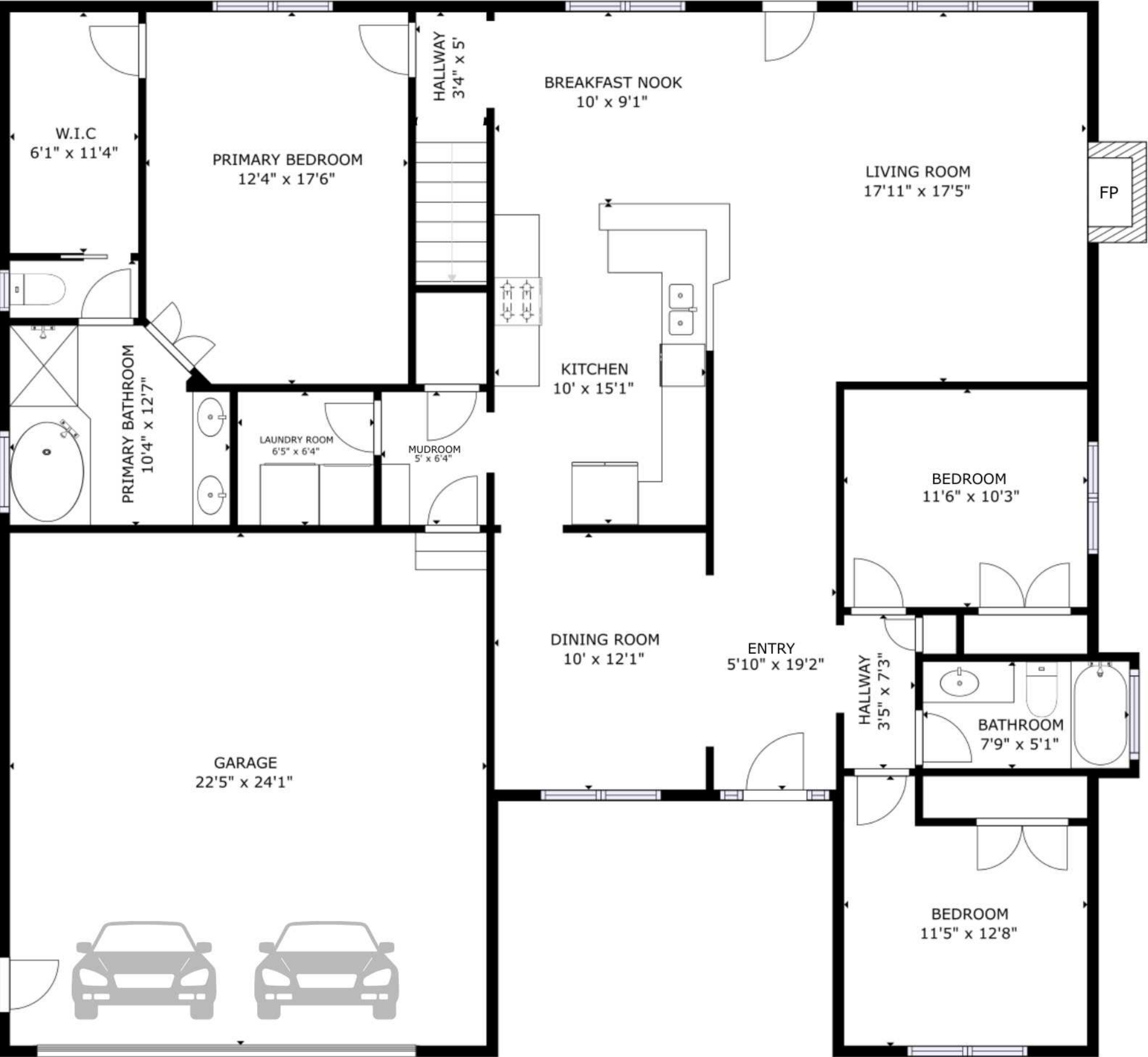
FLOOR 1 1,967 SQ.FT.
