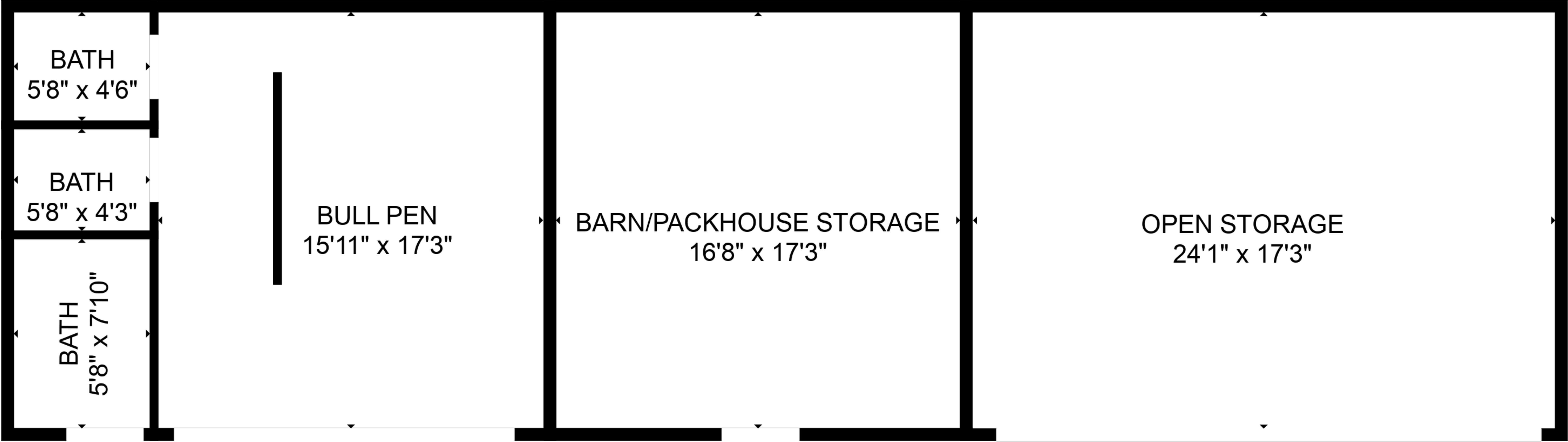
FLOOR 2
