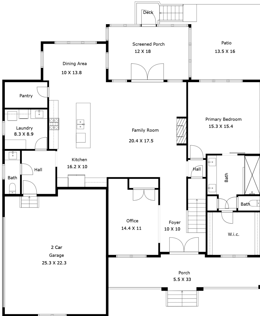
Floor 1
