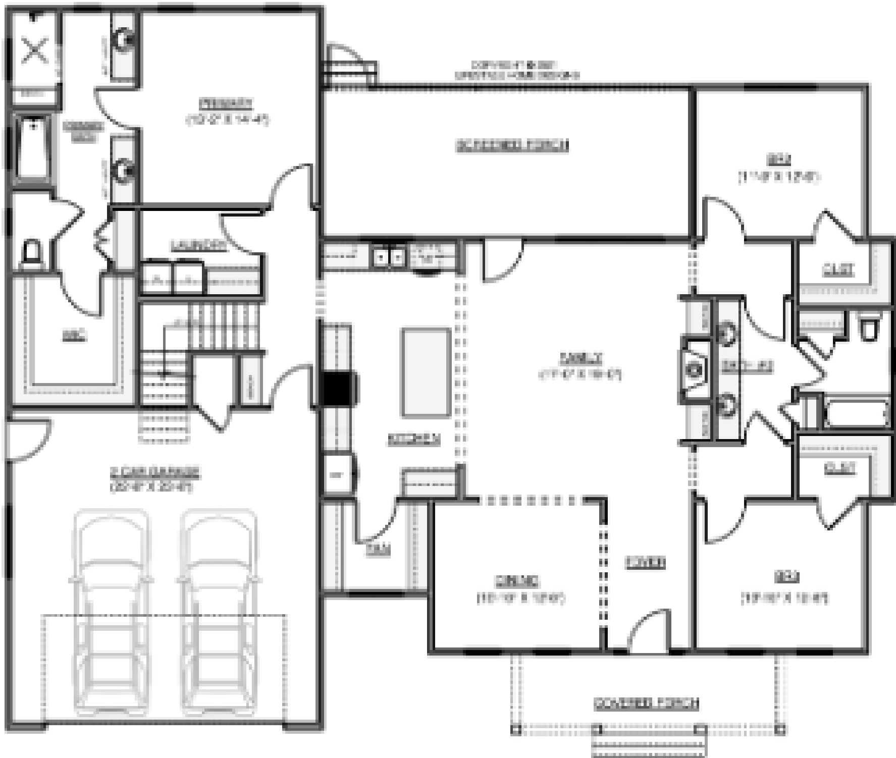
1ST FLOOR
