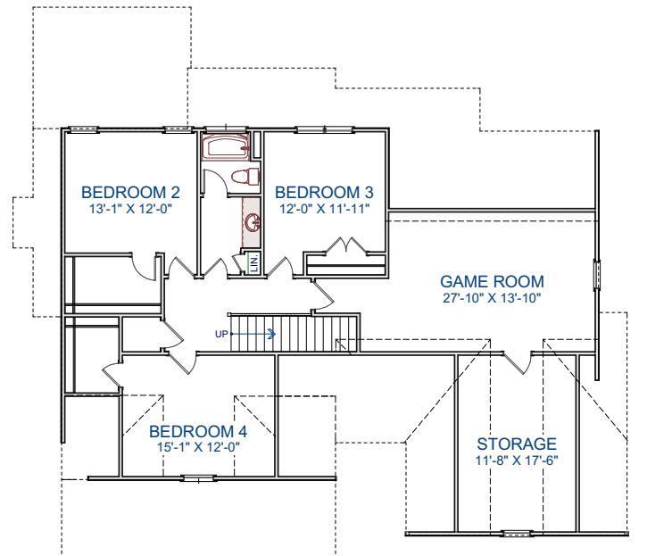
Second Floor
