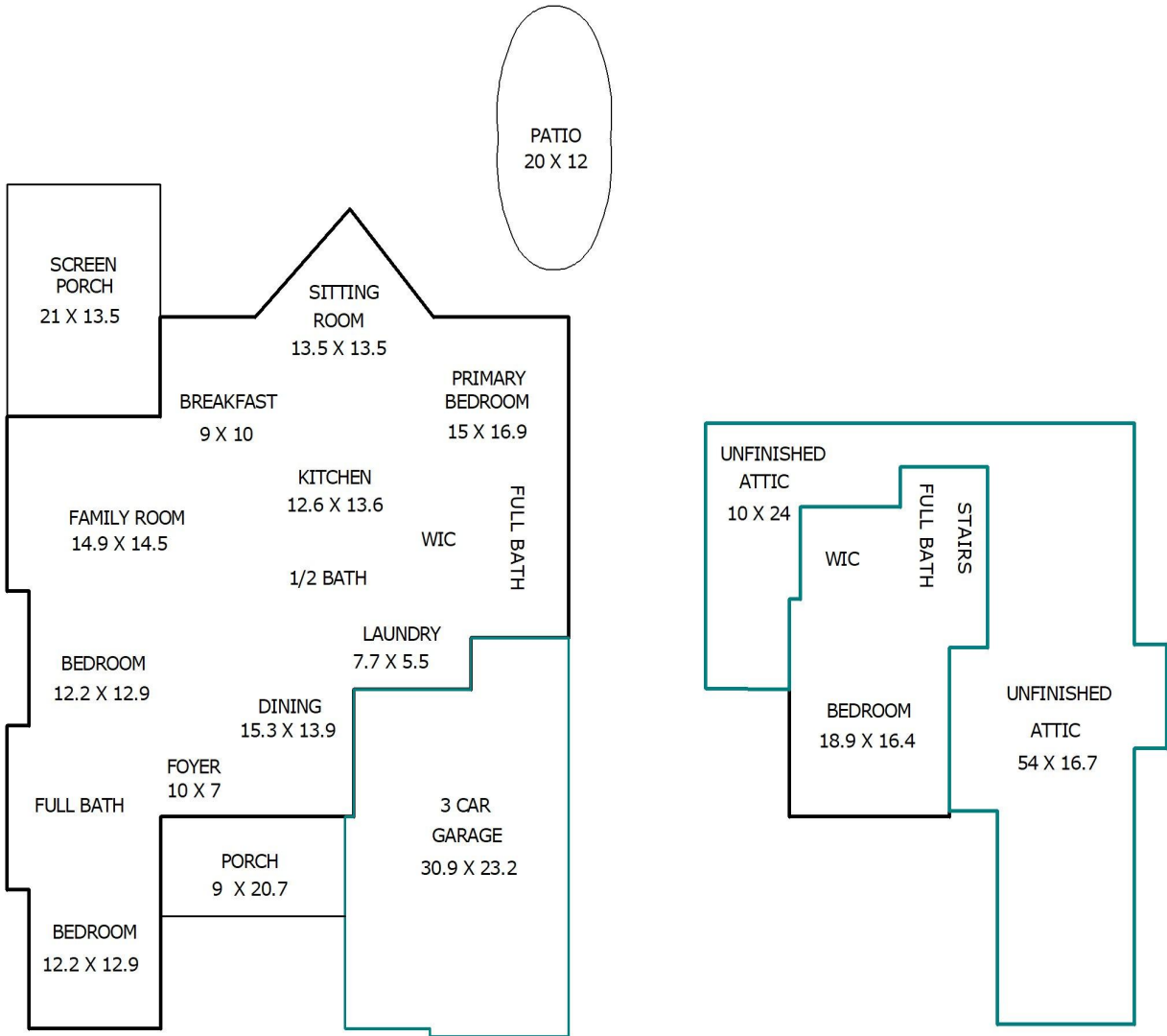
APPROXIMATE DIMENSIONS NOT TO EXACT SCALE
