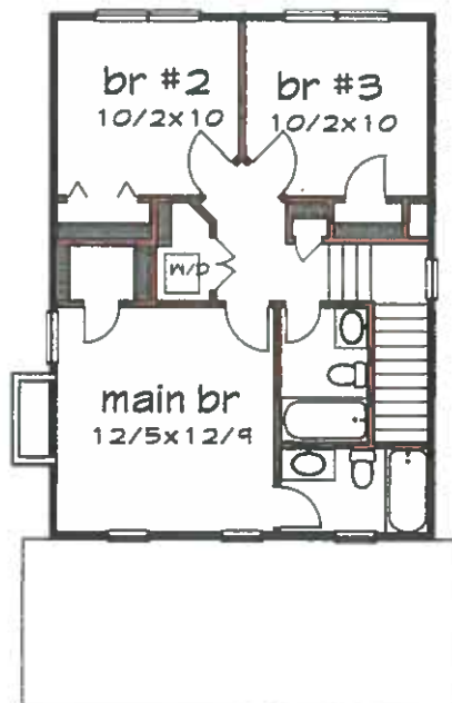
Floor 2 plan
