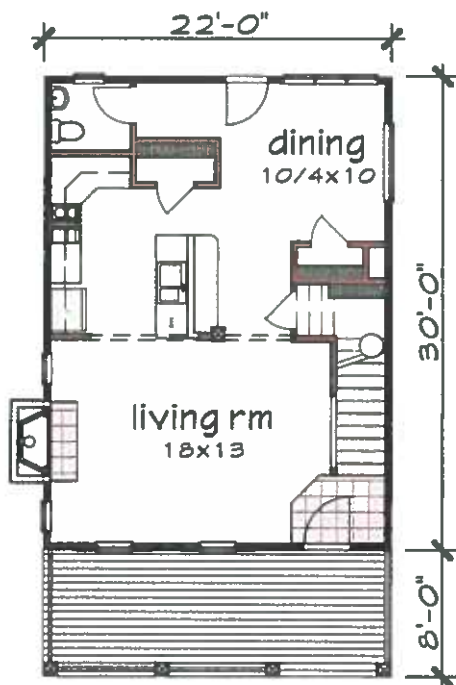
Floor 1 plan
