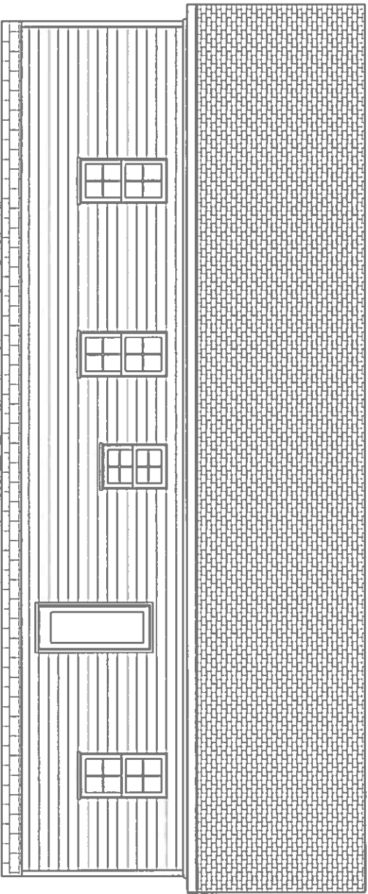
REAR ELEVATION 1/4" = 1'-0"
