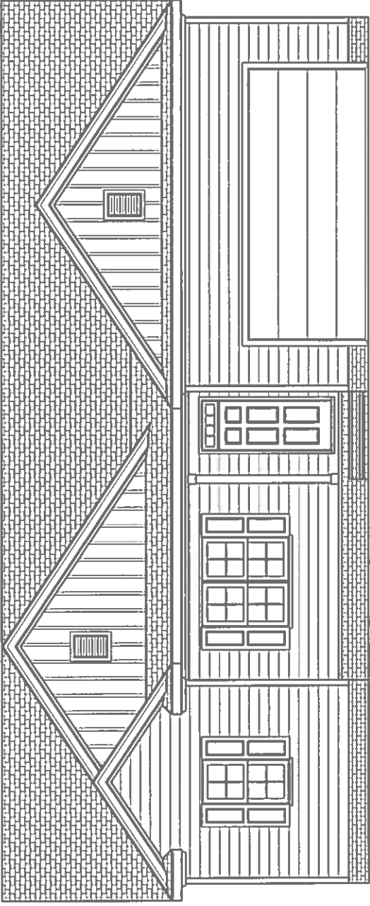
FRONT ELEVATION 1/4" = 1'-0"
